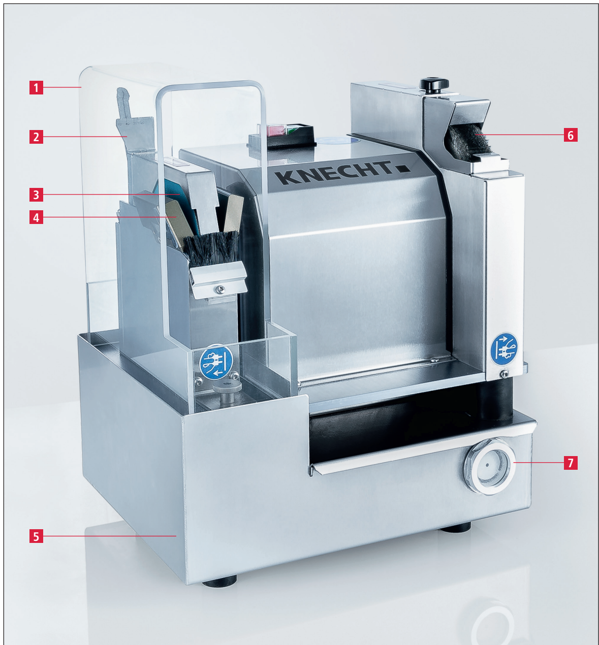
Figure 3-2 Overall view of sharpening machine
