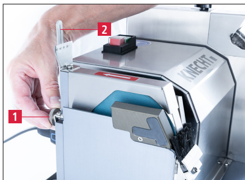
Figure 7-1 Setting the grinding angle
