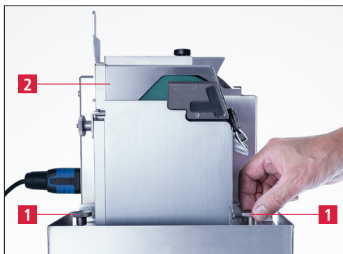
Figure 7-6 Removing knife guide unit
